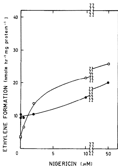
Fig.1. Effect of nigericin and K^+ on the rate of ACC conversion to ethylene in intact mitochondria and in submitochondrial particles; 1.0 ml of the reaction mixture contained 10 mM KCl, 0.1 mM MnCl_2 , 100 mM K-HEPES at pH 8.0 and 190 \mu g of either mitochondrial or submitochondrial protein. Different nigericin concentrations were added after the addition of the membranes. The reaction was started by the addition of 10 mM ACC and ethylene formation was assayed at 20-min intervals, as described in section 2: (○) intact mitochondria; (●) Submitochondrial particles.
